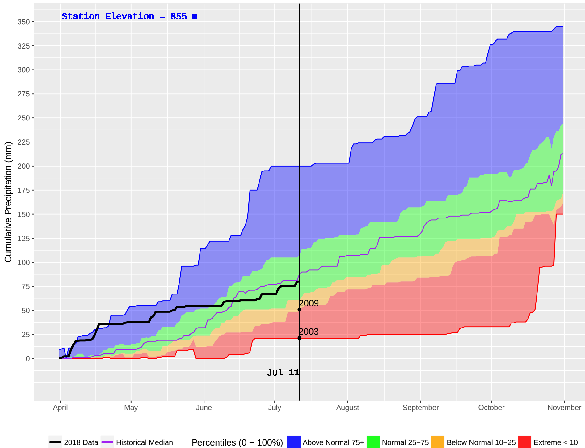
AUGUST LAKE (836) : Historical (2003–2016) and Current (2018) Noon Cumulative Precipitation
