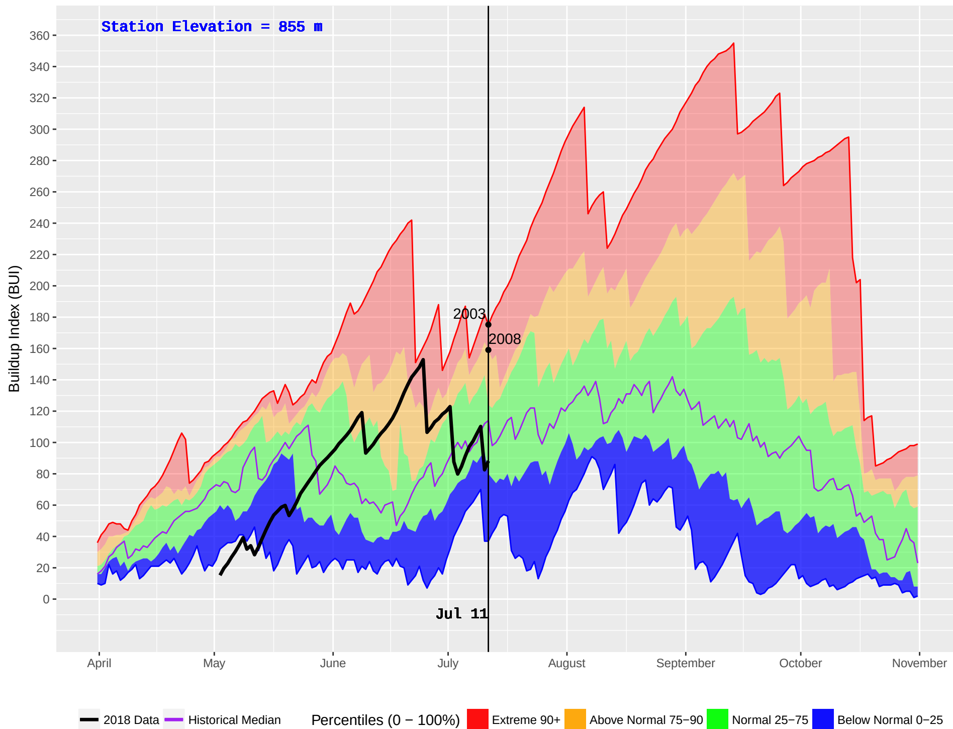
AUGUST LAKE (836) : Historical (2003–2016) and Current (2018) Noon Buildup Index (BUI)
