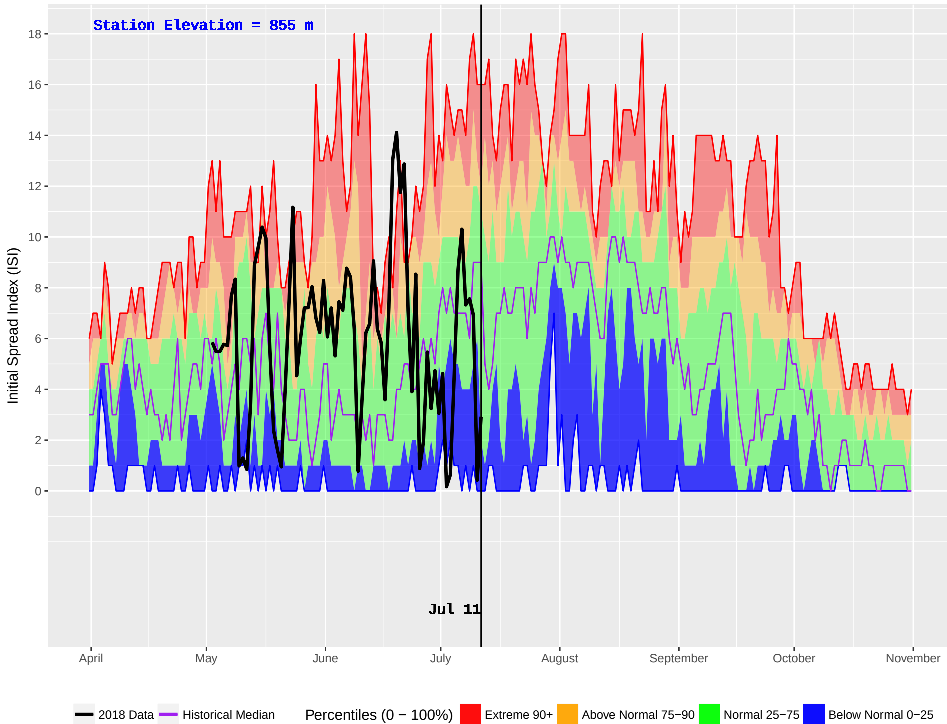
AUGUST LAKE (836) : Historical (2003–2016) and Current (2018) Noon Initial Spread Index (ISI)
