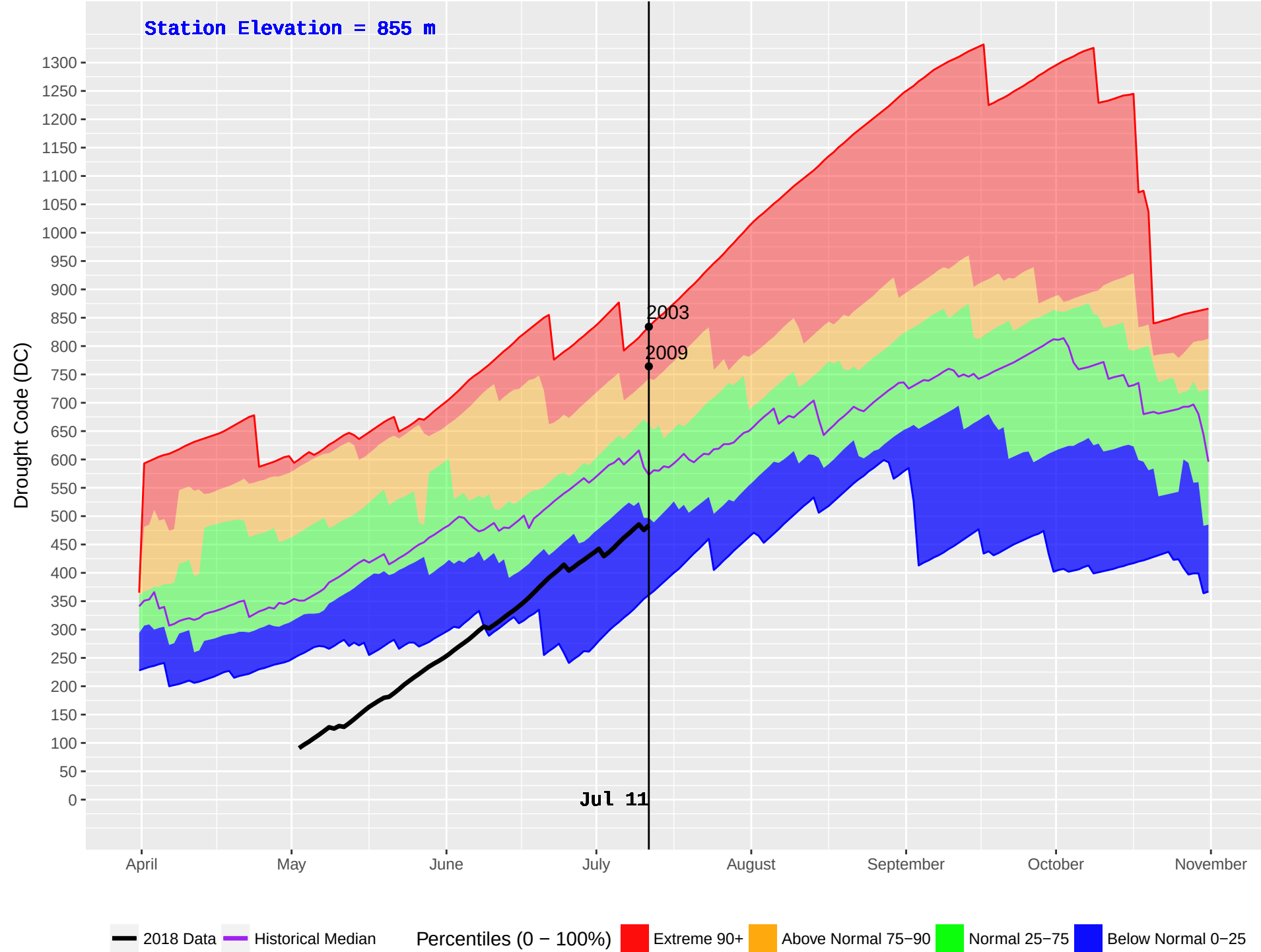
AUGUST LAKE (836) : Historical (2003–2016) and Current (2018) Noon Drought Code (DC)
