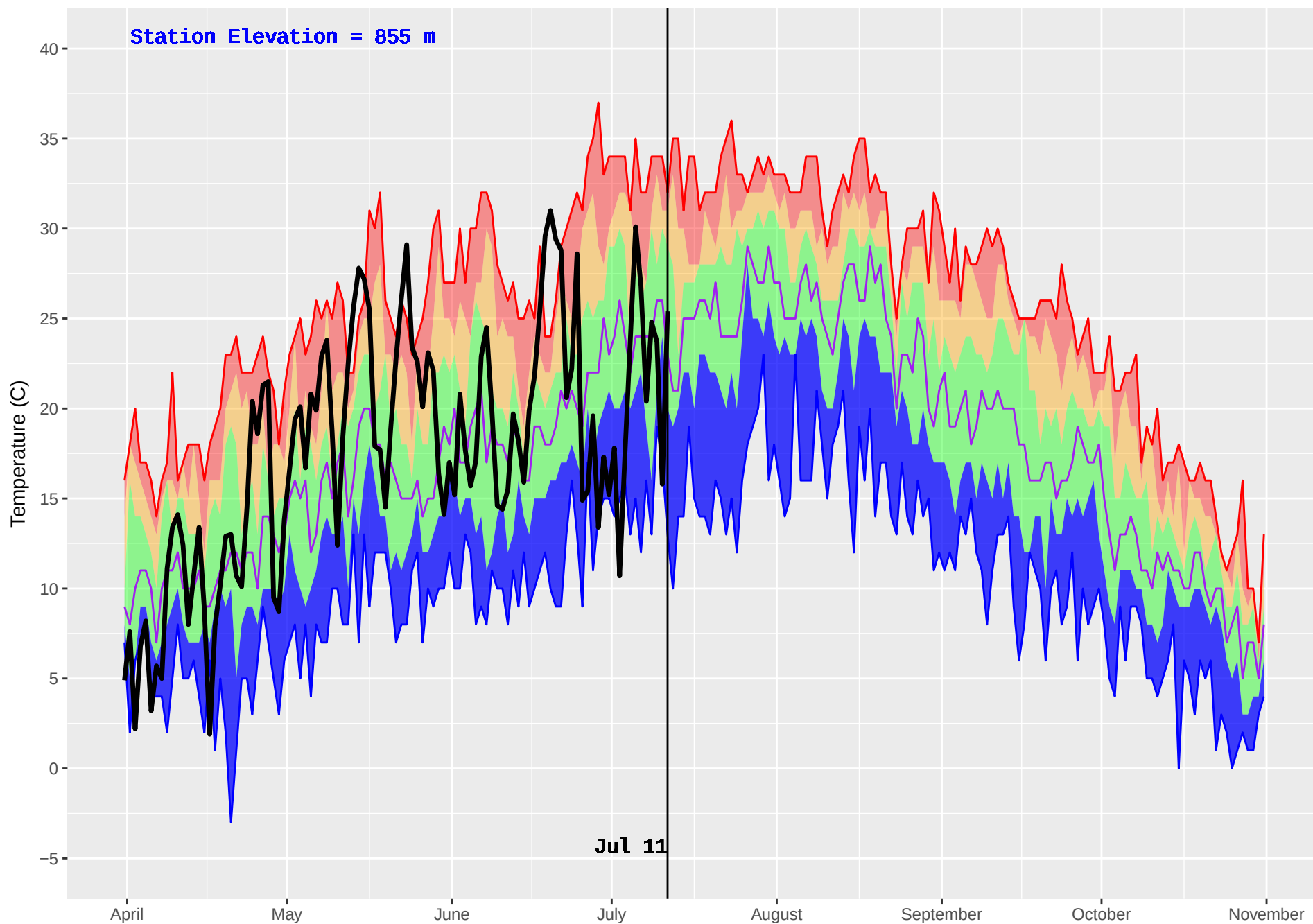
AUGUST LAKE (836) : Historical (2003–2016) and Current (2018) Noon Temperature
